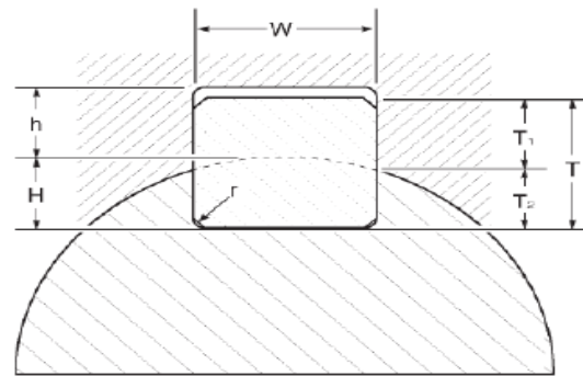
Figure 1 - Keyway and Key Size Dimension Reference
